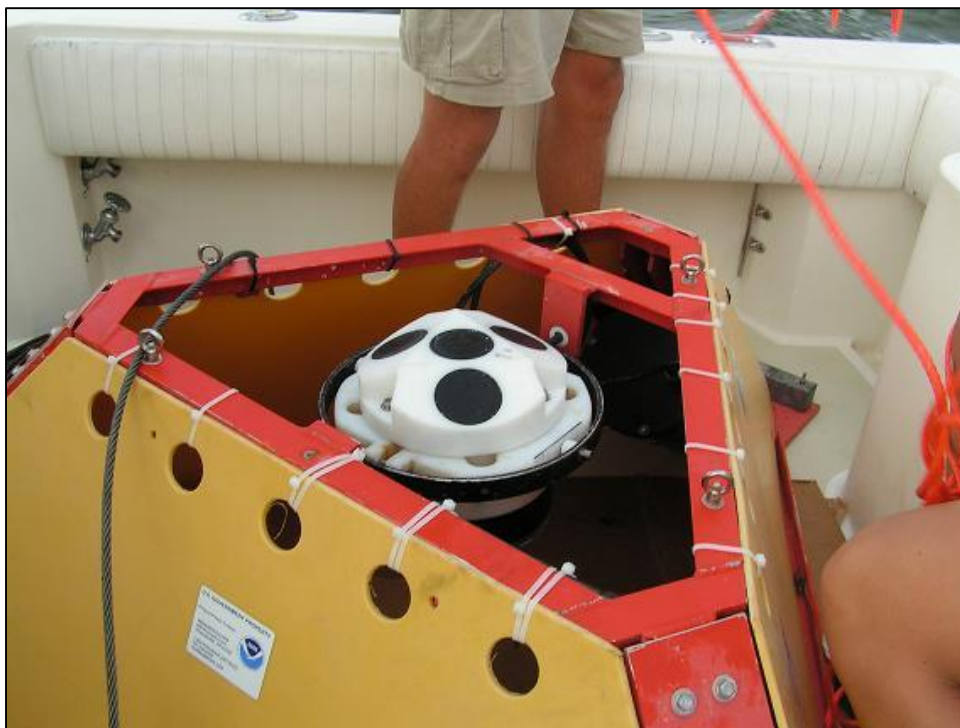
Figure 2-4. Nortek AWAC in a stable, bottom-mounted platform prepared for deployment. (Photo courtesy of Jennifer Patterson/CeNCOOS/Monterey Bay Aquarium Research Institute)
