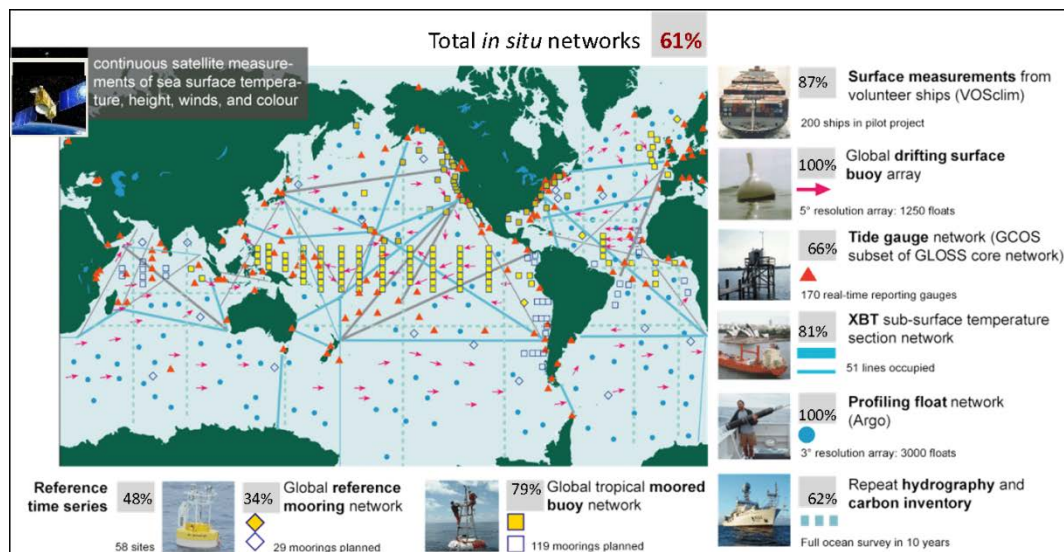
Figure 3. Initial Global Ocean Observing System for Climate
