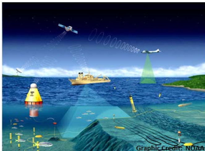
Figure 1. Example of an integrated ocean observation system
