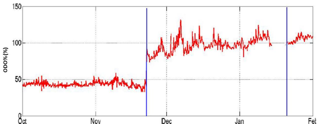
Figure 2-3. Note the abrupt shift in late November 2011 when the badly fouled sensor was replaced. The blue lines indicate the time of sensor replacement. Sensor replacement immediately shows higher saturation percentage. Note also apparent lack of a shift in January 2012 (graphic courtesy of Doug Wilson, NOAA/CBIBS).
