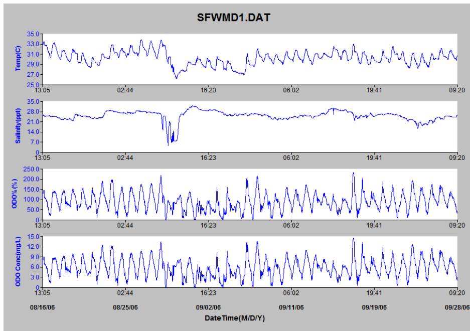
Figure 2-2. Panels 1-4 show temperature, salinity, DO percent, and DO concentration, respectively. The series tracks the passage of a hurricane and the effect it has on the time series before, during, and after the storm front passes (graphic courtesy of Mike Lizotte, YSI).
